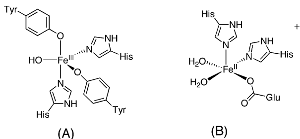
Figure 7. Iron coordination environment in (A) intradiol and (B) extradiol dioxygenases.
